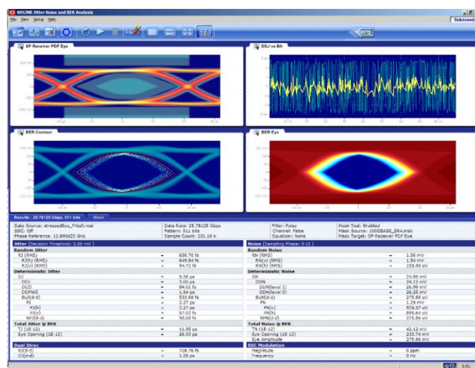
Jitter, noise and BER analysis
