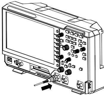
Figure 6 To Connect the Passive Probe
