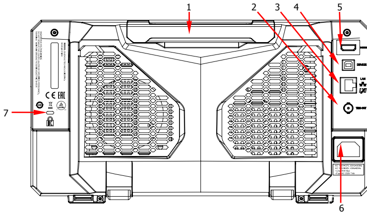
Figure 2 Rear Panel
