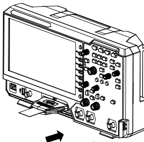
Figure 7 To Connect the Logic Probe
